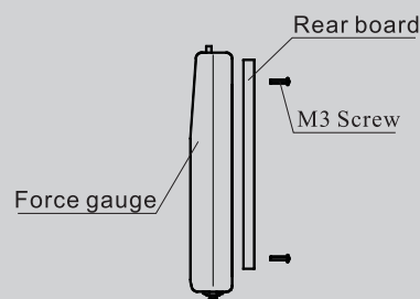
Installation figure of force gauge
