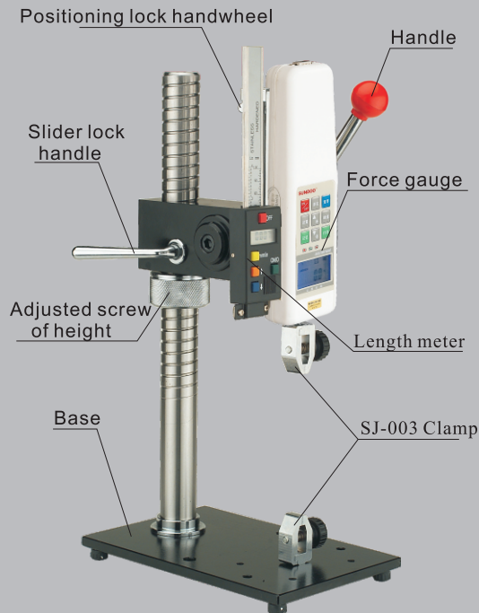
SPJ-B Manual test stand
