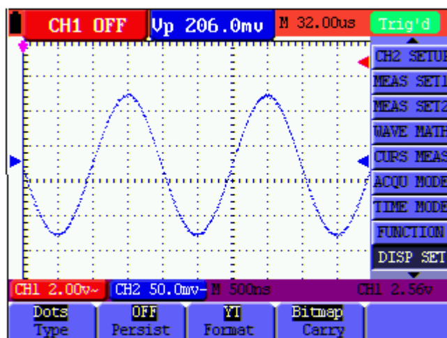
Figure 46: Dots Style
